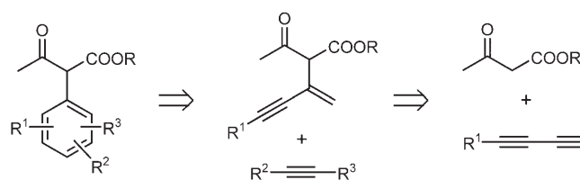
Figure 1. A modular approach to \alpha -arylated carbonyl compounds.
